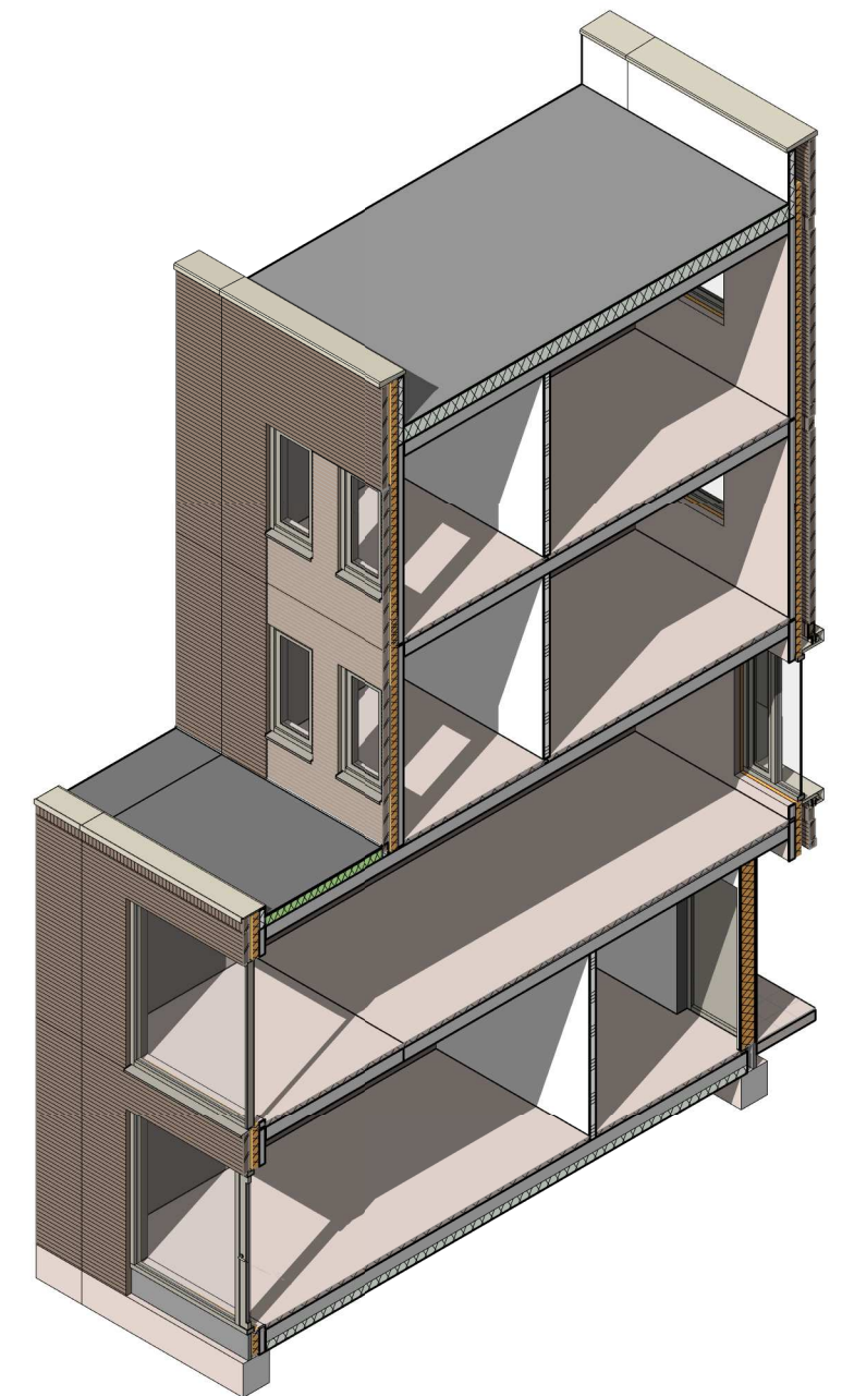
3D isometrie
